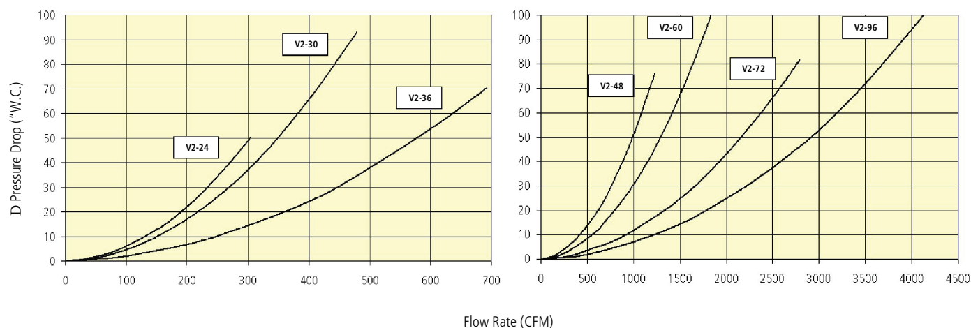
Pressure Drop Graph for V2 Series Vessels
